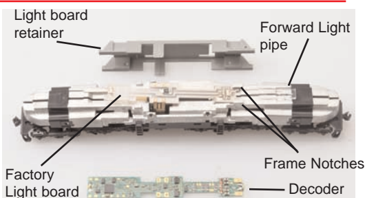
Figure 1: Remove loco shell and lightboard retainer
